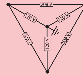
208 V WYE
