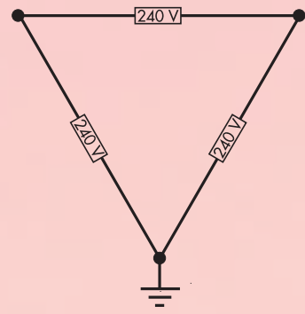
240 V Delta Corner Ground
