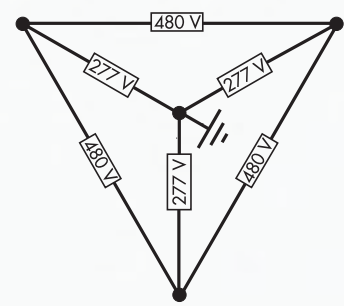
480 V WYE
