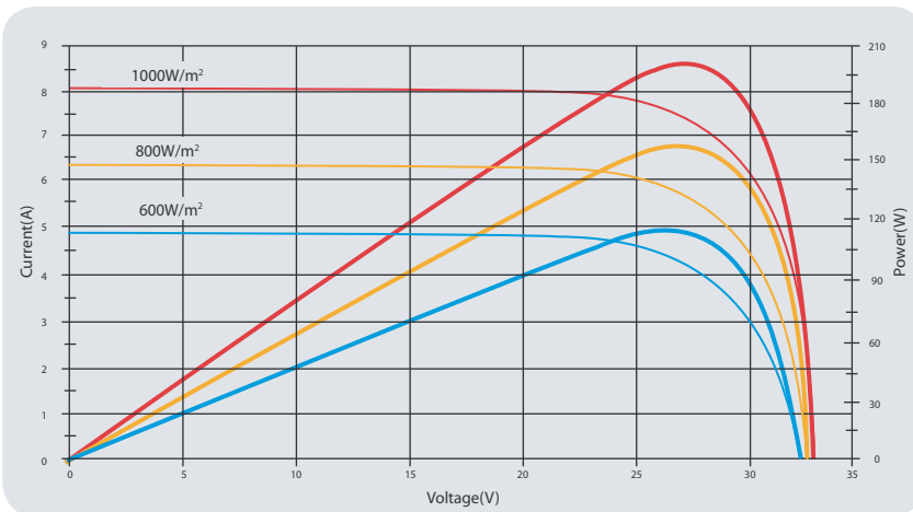
Current-Voltage & Power-Voltage Curve (200W)
