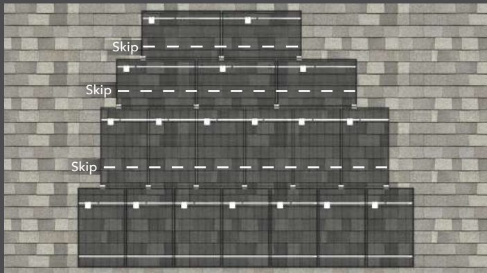
Example of Comp Roof Array
