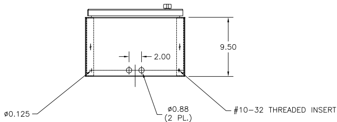
BOTTOM (STRUT NOT SHOWN)
