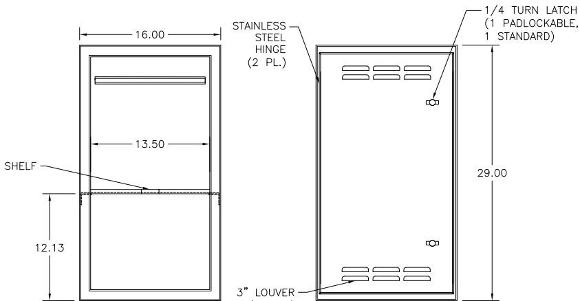
FRONT (DOOR NOT SHOWN)
