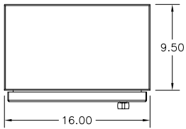
TOP (STRUT NOT SHOWN)
