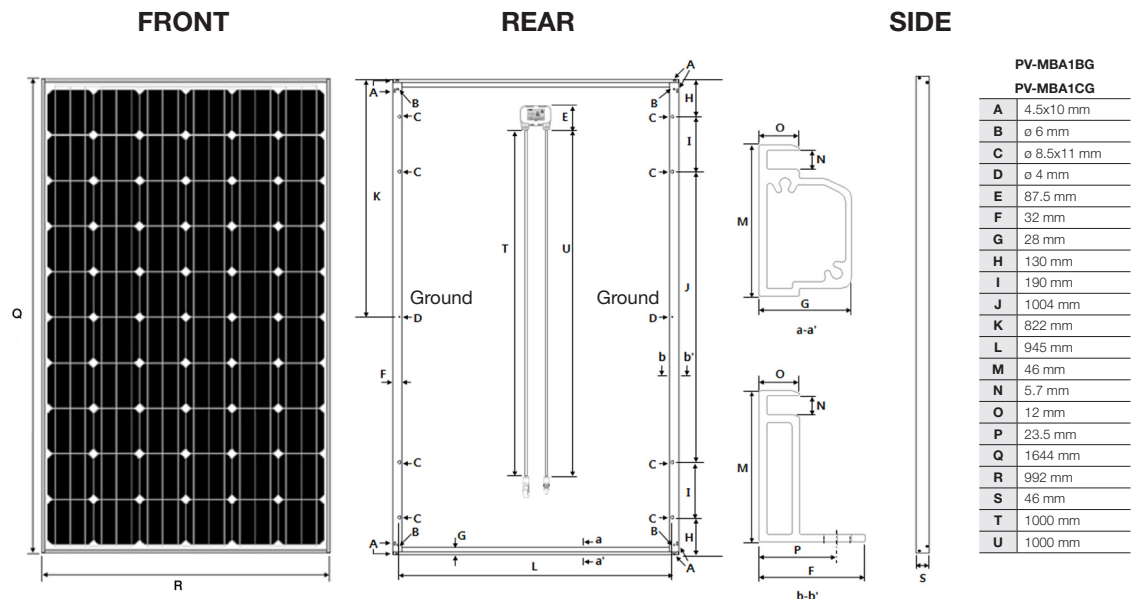
Figure 1 - Dimension of PV Module (PV-MBA1BG / PV-MBA1CG)
