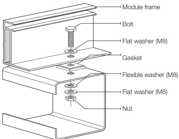
Figure 3 - Module mounting method
