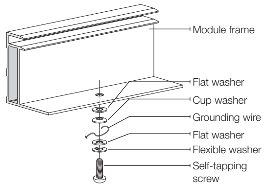
Figure 2 - Grounding method 2 using self-tapping screw
