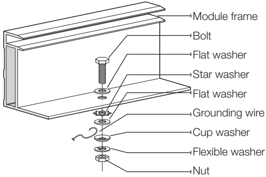
Figure 2 - Grounding method 1 using bolt and nuts
