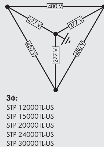
480 V WYE
