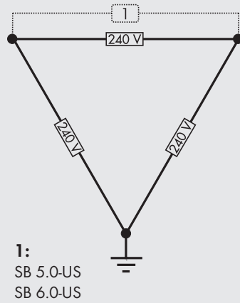
240 V Delta Corner Ground
