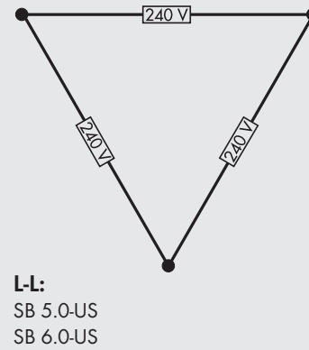
240 V Delta
