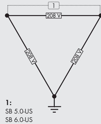
208 V Delta Corner Ground
