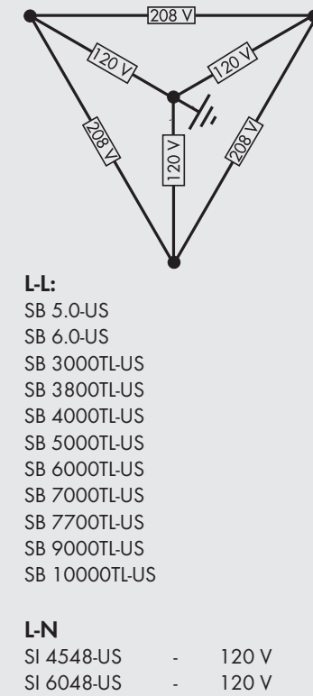
208 V WYE
