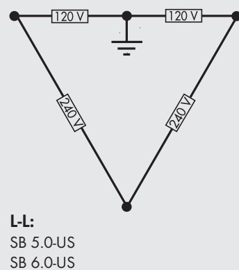
240 V Stinger Ground
