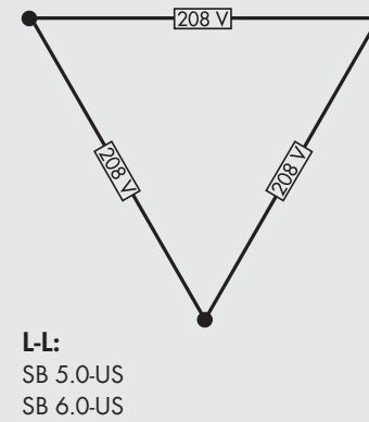
208 V Delta
