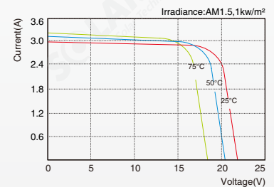
SLP045-12 I-V Curves
