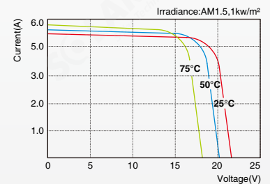
SLP090-12 I-V Curves
